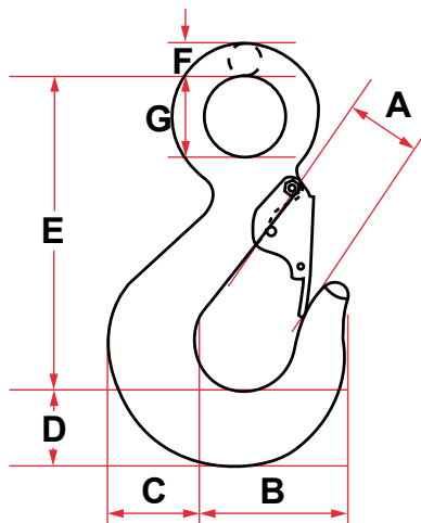
STANDARD HOOK WITH SAFETY LATCH
