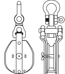
Steel Shell Block with Drilled Swivel Eye & Shackle
