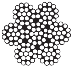
TYPICAL STRAND CORE (SC)
