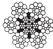
TYPICAL INDEPENDENT WIRE ROPE CORE (IWRC)
