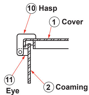
DETAIL OF HASP & EYE
