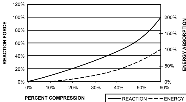
GENERIC PERFORMANCE CURVE OCEAN GUARD FENDER
